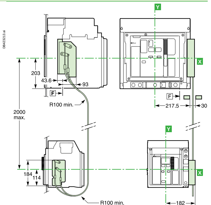
Drawout Devices
