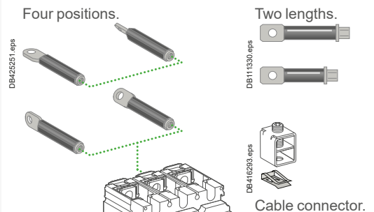
Cable connector.
