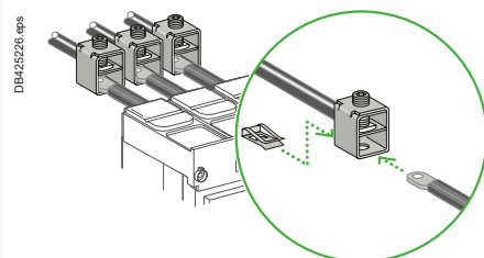
Connection of bare cables to NSX100 to 250 by clips.
