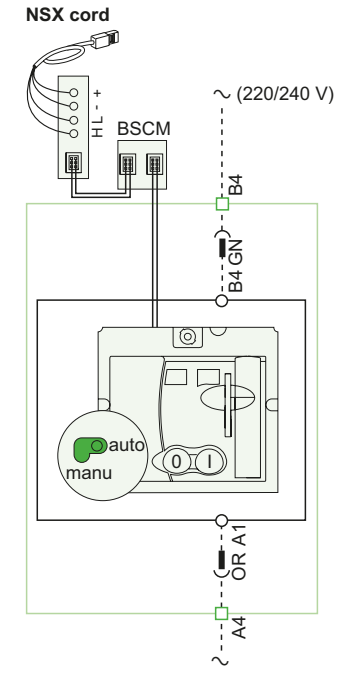
Communicating motor mechanism (MTC)
