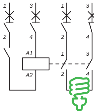
Layout with power relay
