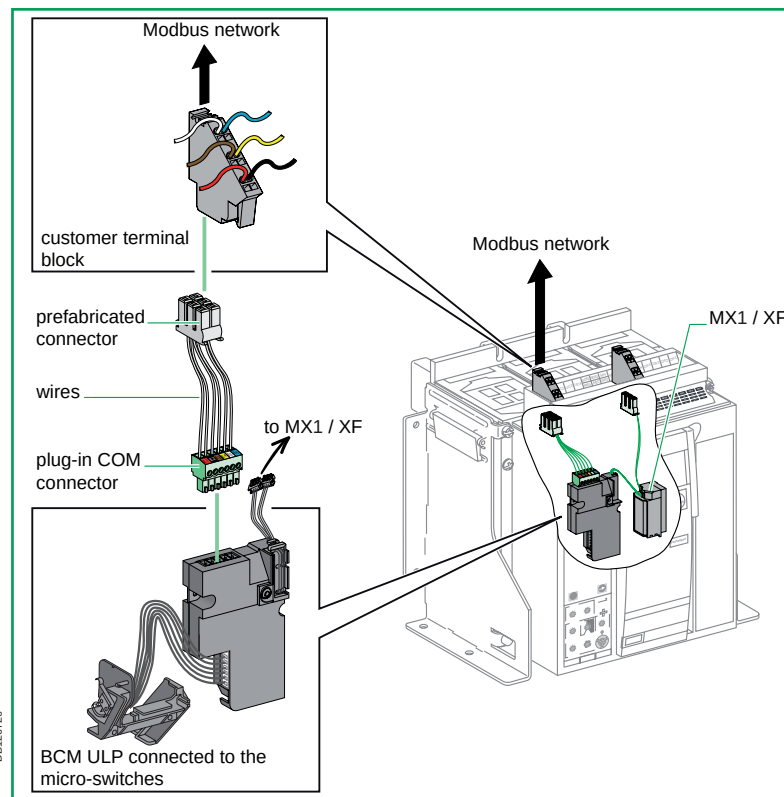
Modbus BCM ULP "device" communication module installation on a fixed, electrically operated Compact NS or Masterpact NT/NW.
