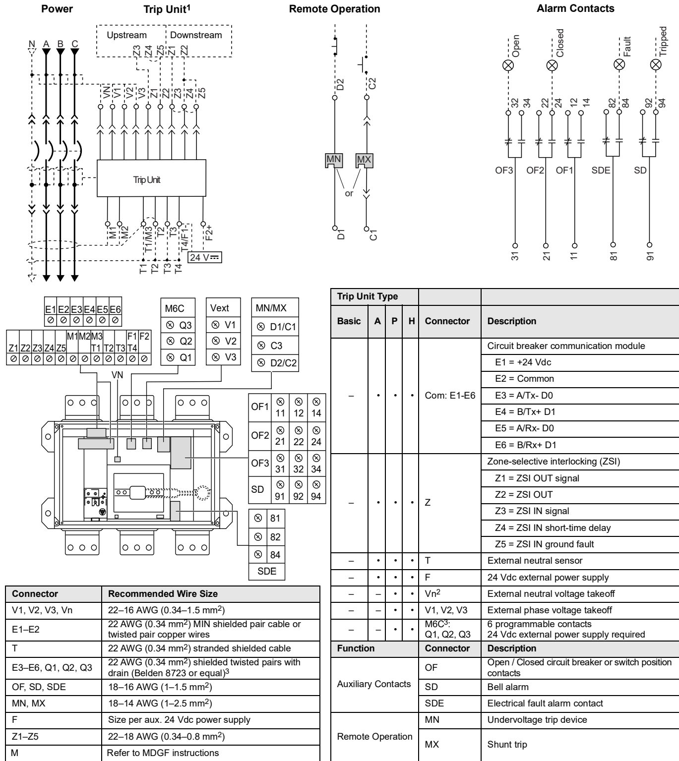
FIG. 2 : Accessory Control Wiring Diagram (English)
